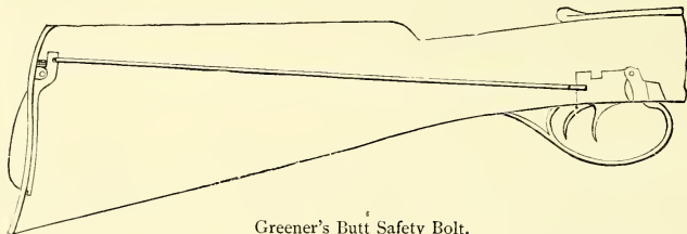
Greener's Butt Safety Bolt.
